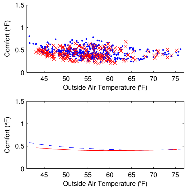
Fig. 8. The cross marks and solid line (points and dashed line) denote the comfort characteristics of the LBMPC (default) controller.
