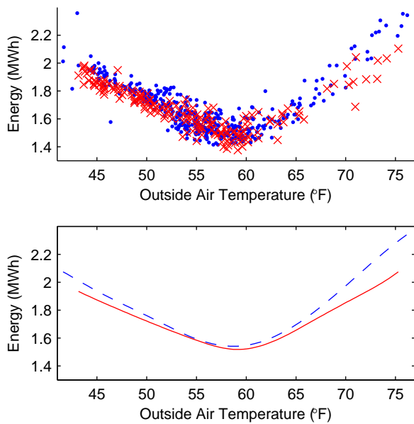
Fig. 7. The cross marks and solid line (points and dashed line) denote the energy characteristics of the LBMPC (default) controller.
