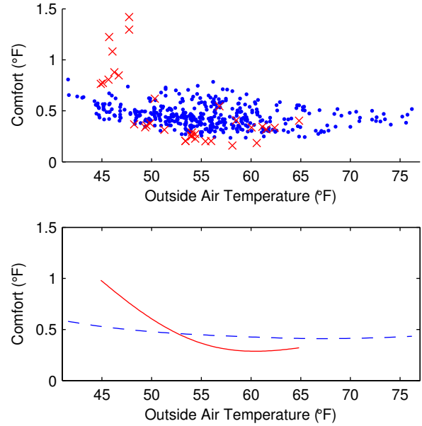
Fig. 6. The cross marks and solid line (points and dashed line) denote the comfort characteristics of the schedule (default) controller.
