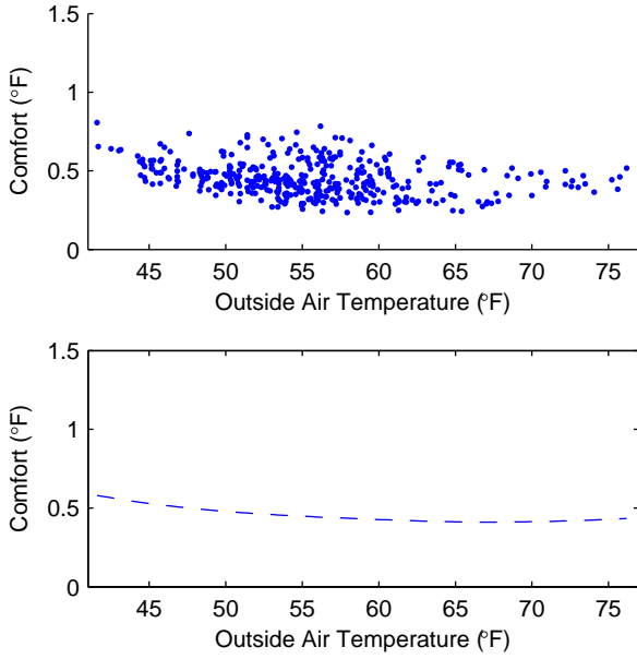
Fig. 3. The scatter plot shows the data points (T_0[i], C[i]) , and the smooth curve is the estimated comfort characteristic \hat{C}_{o,x}(T_0) for an HVAC controller.
