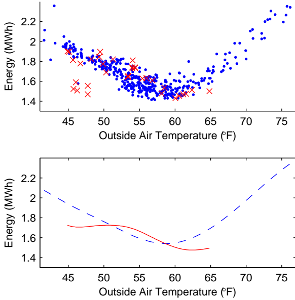
Fig. 5. The cross marks and solid line (points and dashed line) denote the energy characteristics of the schedule (default) controller.
