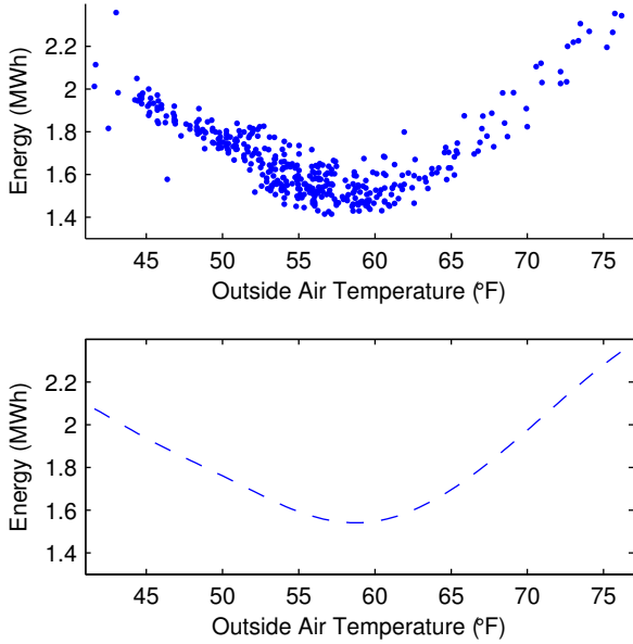
Fig. 1. The scatter plot shows the data points (T_o[i], E[i]) , and the smooth curve is the estimated energy characteristic \hat{E}_{o,x}(T_o) for an HVAC controller.
