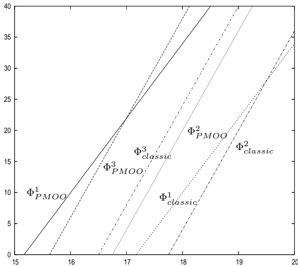
Figure 5: Service curves of paths.
