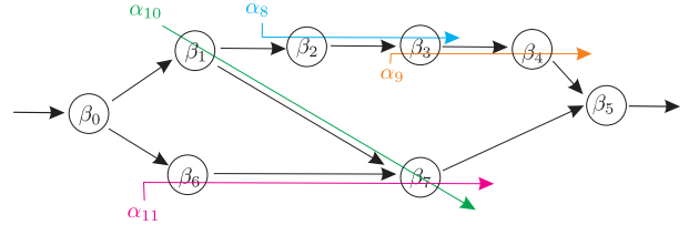
Figure 4: An example of a strongly acyclic network.
