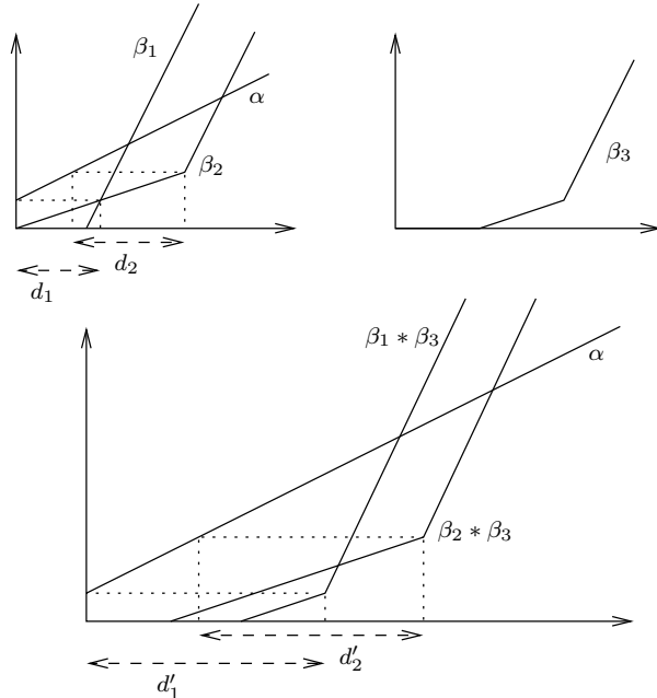
Figure 2: No subpath optimality property for delays.
