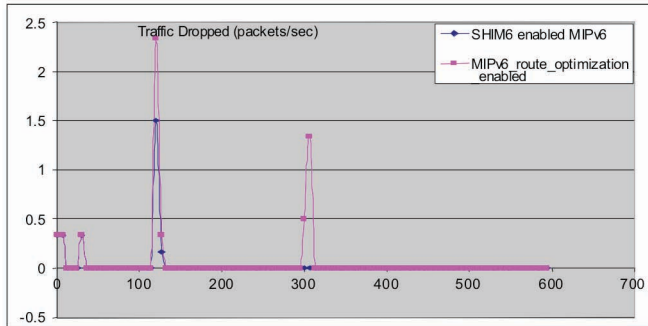
Figure 9. Traffic Dropped.
