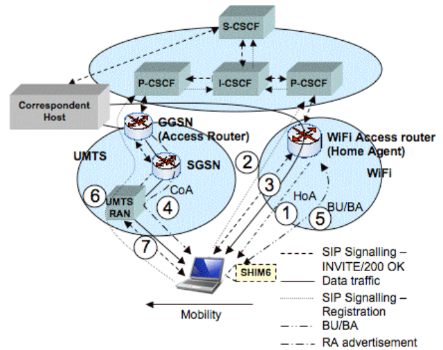
Figure 3. Mobile IPv6 Support for IMS architecture interaction process.
