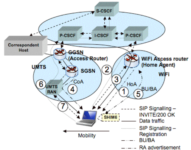
Figure 5. SHIM6 support for IMS architecture interaction process
