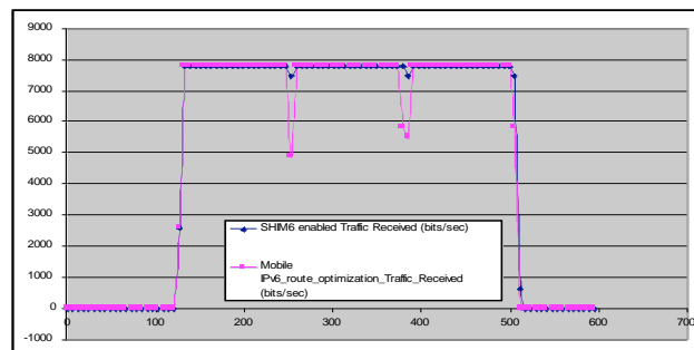
Figure 8. Traffic Received.
