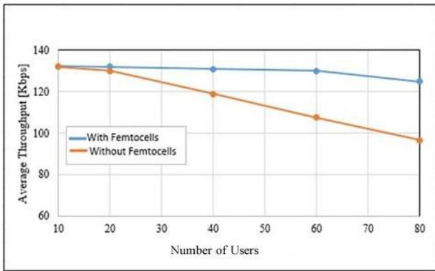
Figure 5. Average Throughput per flow
