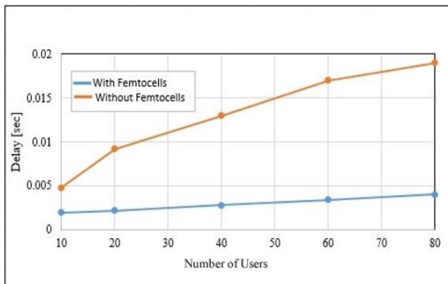
Figure 6. Delay for video flows
