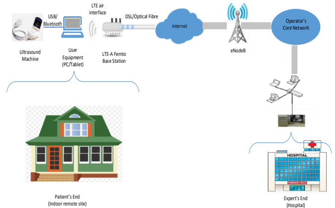
Figure 1: Indoor medical ultrasound streaming scenario.
