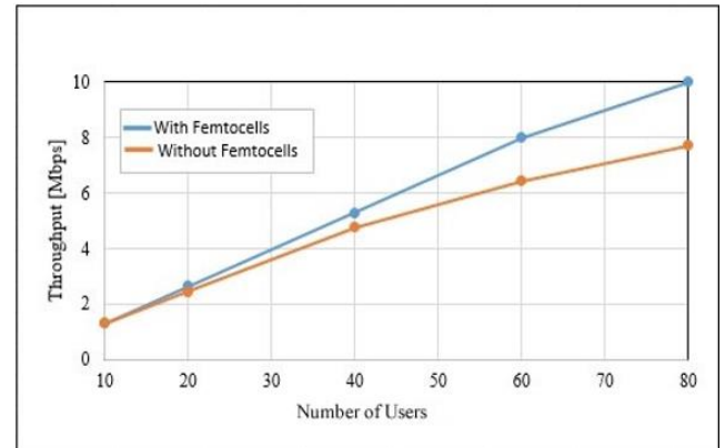
Figure 4. Aggregated Throughput.
