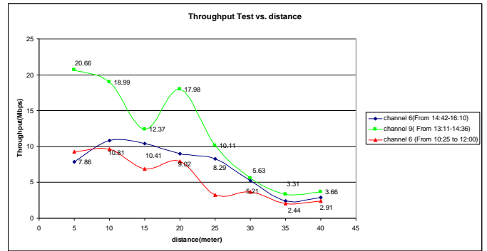
Fig. 1. Throughput of a four-node Wi-Fi IEEE 802.11g network as a function of network radius (congested outdoor environment, all terminals at line-of-sight and RSSI always > -70 dBm) [17]
