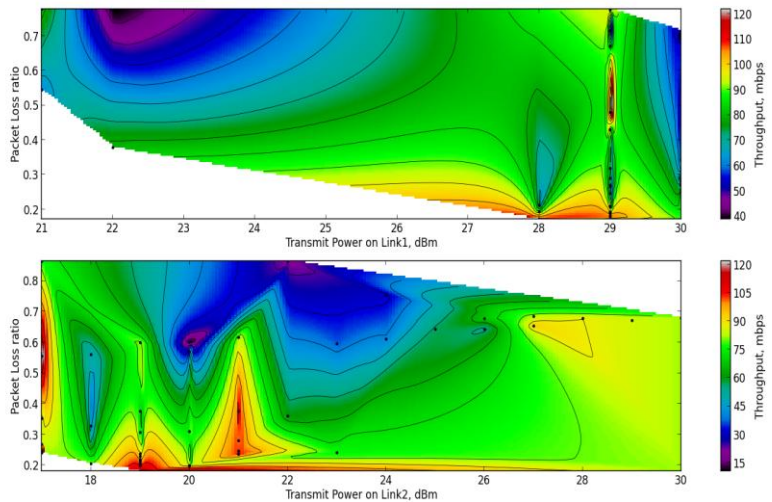
Fig. 9. Transmit power and throughput with different loss on Link1 and Link2
