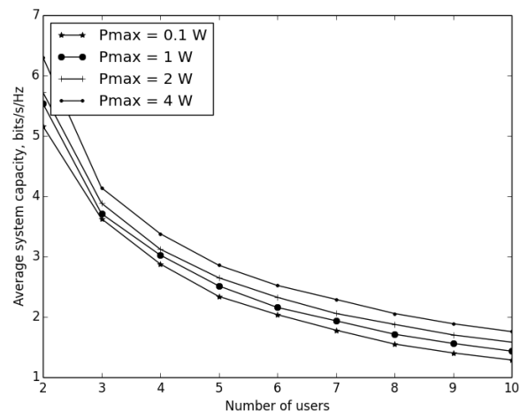
Fig. 3. Average link capacity in the simulated system as function of total number of users
