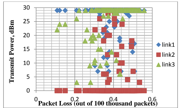
Fig. 5. Packet loss distribution at different transmit power levels on three experimental links
