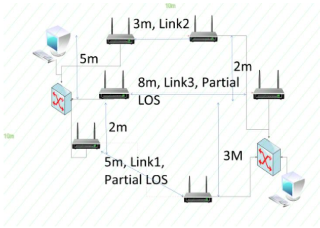
Fig. 4. The experimental setup for testing power coordination algorithm
