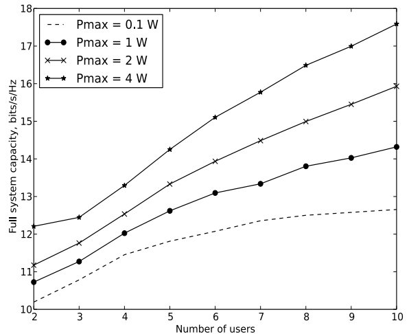
Fig. 2. Total system capacity for simulated devices with interference-aware power control game ( 100 \times 100 m area, frequency 5500 MHz)
