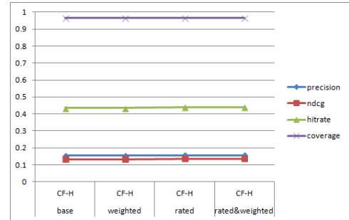
Fig. 12. Results for different settings: CF-H
