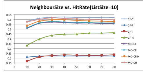
Fig. 4. N vs Hitrate when k = 10
