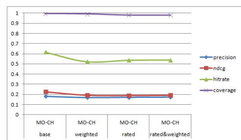
Fig. 16. Results for different settings: MO-CH
