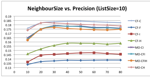
Fig. 3. N vs Precision when k = 10
