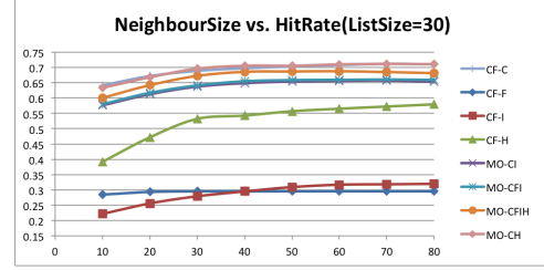
Fig. 6. N vs Hitrate when k = 30
