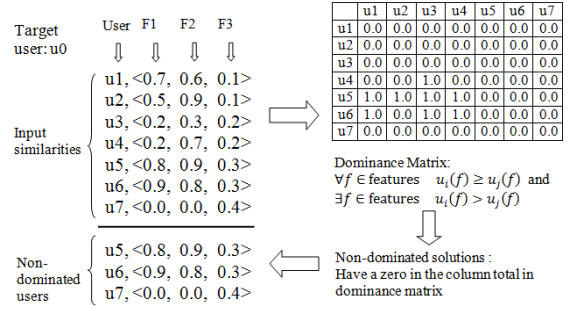
Fig. 2. Example input and non-dominated solutions
