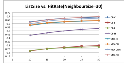
Fig. 8. k vs Hitrate when N = 30
