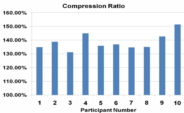
Fig. 9. The compression ratio of the delta algorithm.
