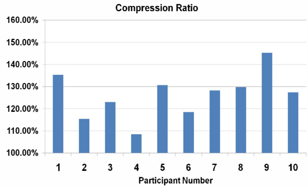
Fig. 10. The compression ratio of the Huffman algorithm.
