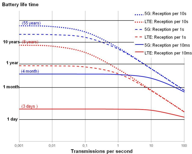
Fig. 8. Battery life time comparison for M2M optimized LTE and 5G.
