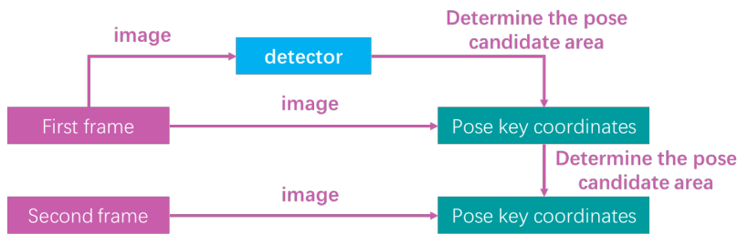
Figure 1. Flowchart of Blaze-Pose reasoning
