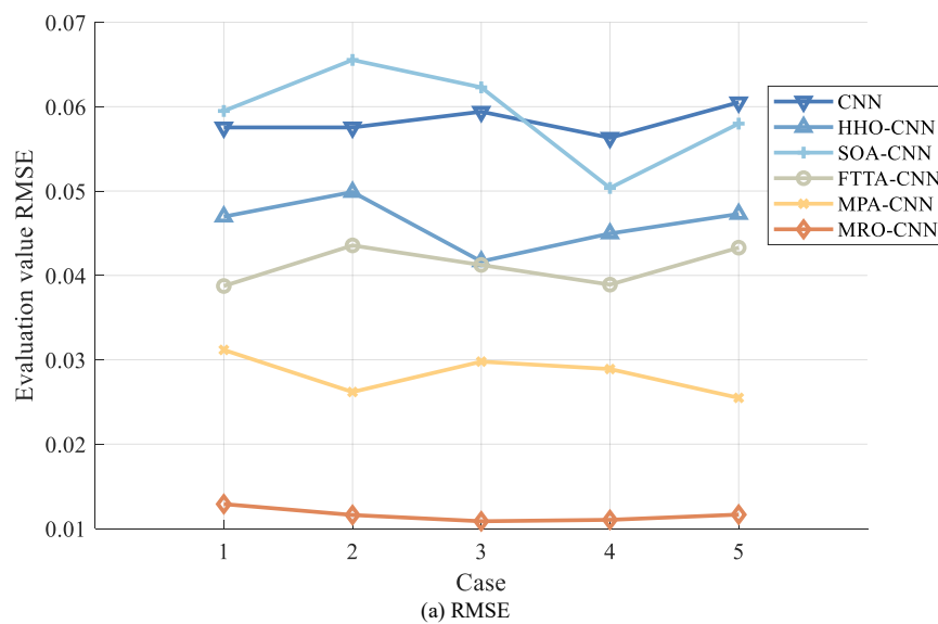
(a) RMSE
