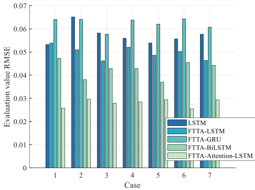
(a) RMSE
