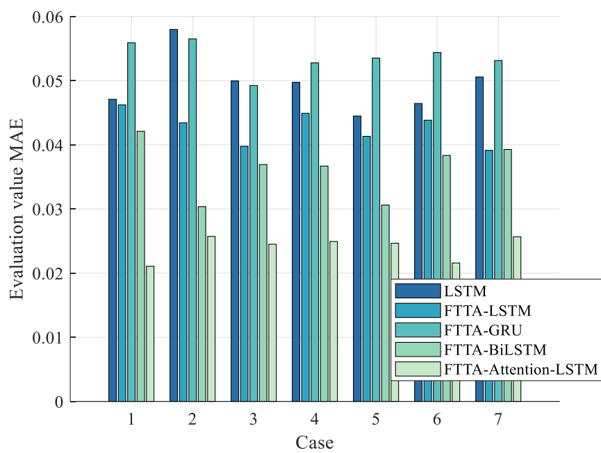
(c) MAE
