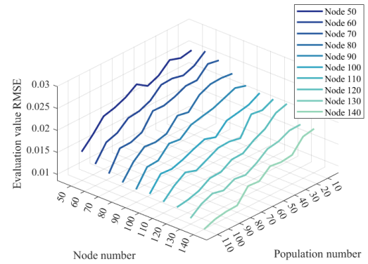
Figure 10. Different population sizes and different hidden layer node conditions on the accuracy of analysing the physical fitness-specific training patterns of basketball teams
