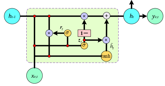
Figure 4 GRU network
