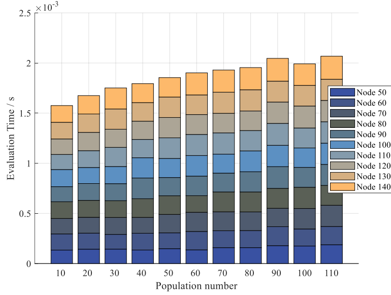
Figure 9 Analysis time for different population sizes and number of CNN hidden layer nodes
