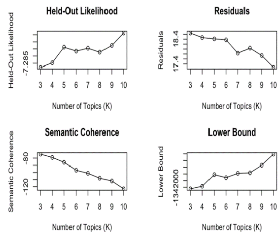
Figure 8. Diagnostic Plot for K
