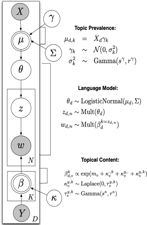
Figure 1. Plate Diagram for the Structural Topic Model
