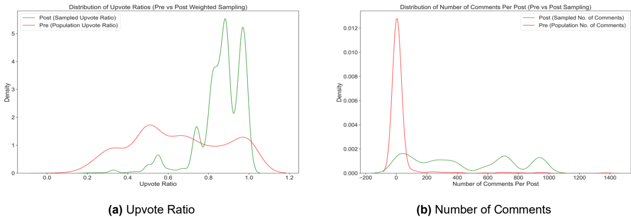
Figure 3. Pre vs Post Weighted Sampling Comparison of Feature Based Distribution
