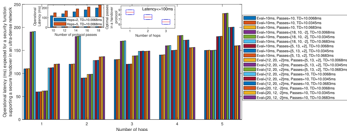
Figure 4. Understanding the expected impact on secure handover latency in terms of operational activity of a security function for 6G networks with variation in the number of hops, evaluation time (Eval), number of protocol passes (Passes), and one-way packet transportation delay (TD).
