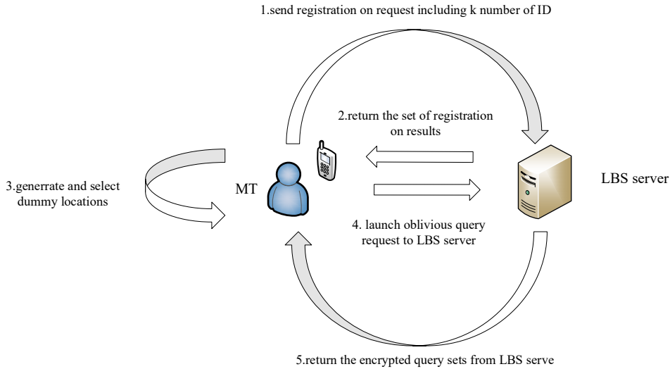
Figure 1. Architecture of location privacy protection system in this scheme
