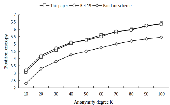
Figure 4. The relationship between anonymity degree K and position entropy
