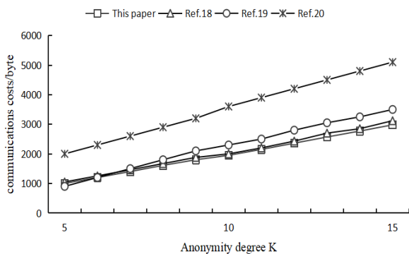
Figure 2. The relationship between degree of anonymity K and communications costs
