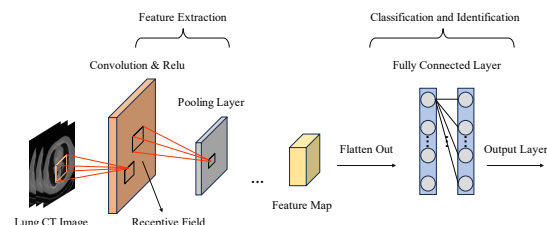
Figure 4. The general structure of CNN
