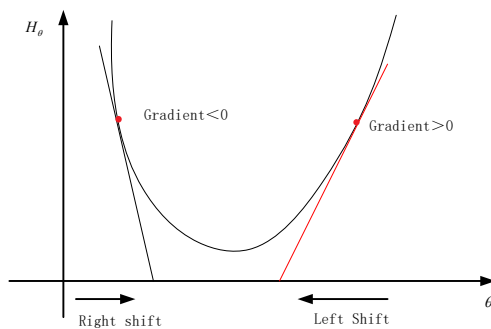
Figure 7: Stochastic Gradient Descent (SGD)
