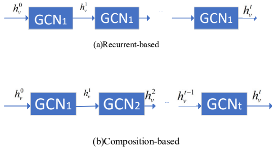
Figure 4: Comparison of Recurrent-based and Composition-based method in spatial-based GCN
