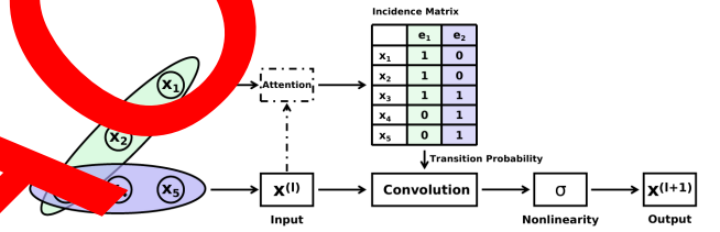
Figure 6. Attention Mechanism [33]
