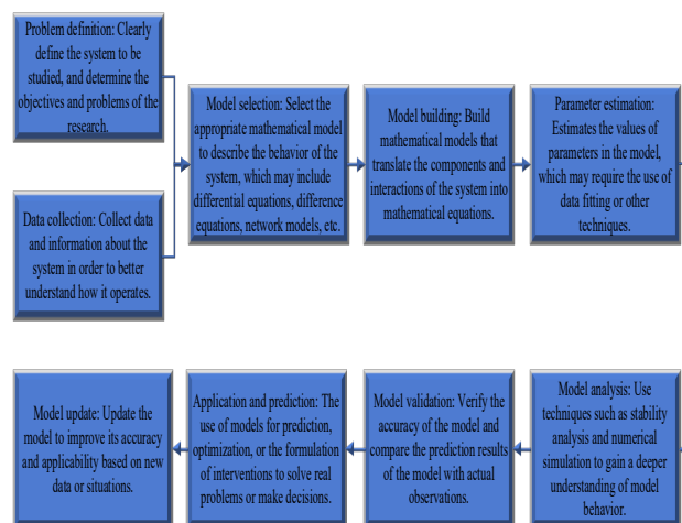
Figure 1. The mathematical modeling process of complex systems
