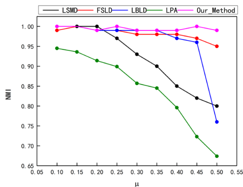
Figure 5. NMI comparison on artificial data set
