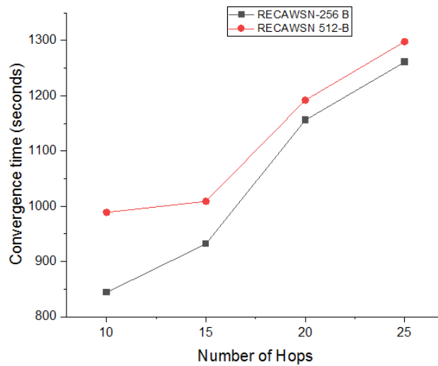
Fig.4 Number of hops versus Convergence time
