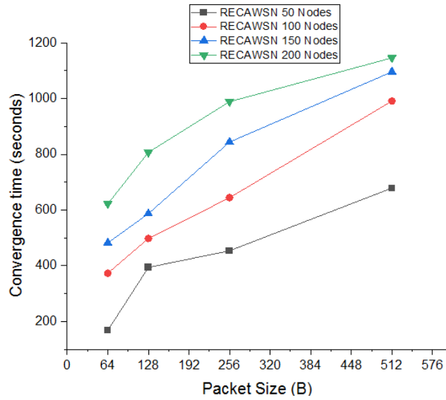
Fig.3 Packet size versus Convergence time
