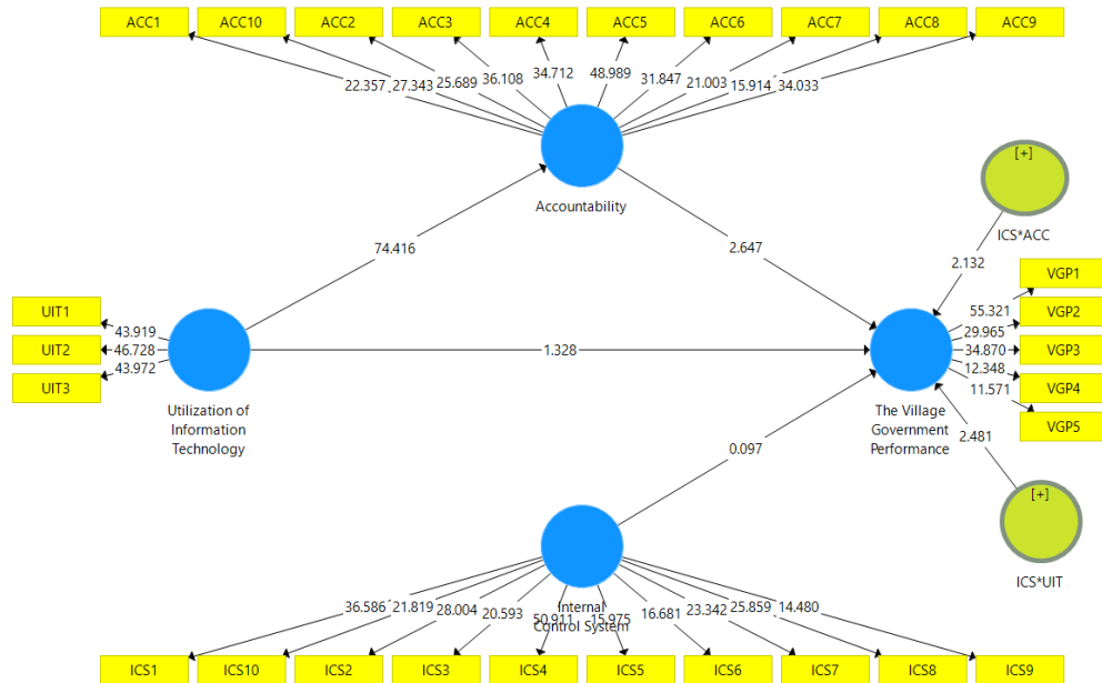
Fig. 3. Inner model result (bootstrapping)
