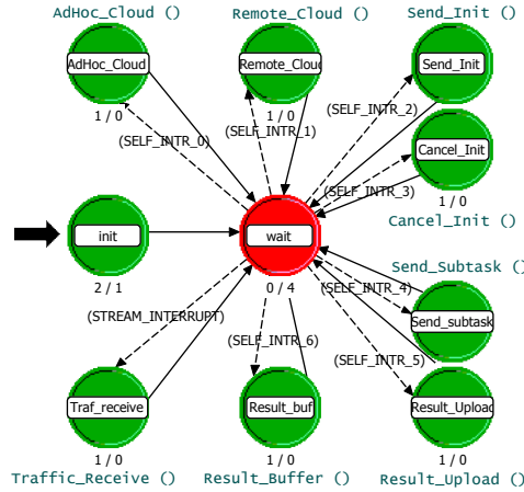
Fig. 3. Computation offloading process model.
