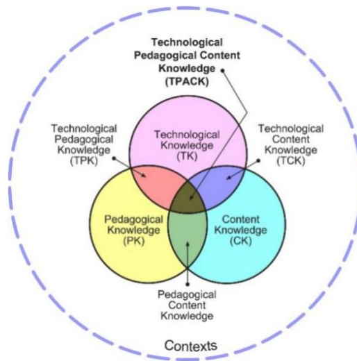
Fig. 1. TPACK Framework [2].
