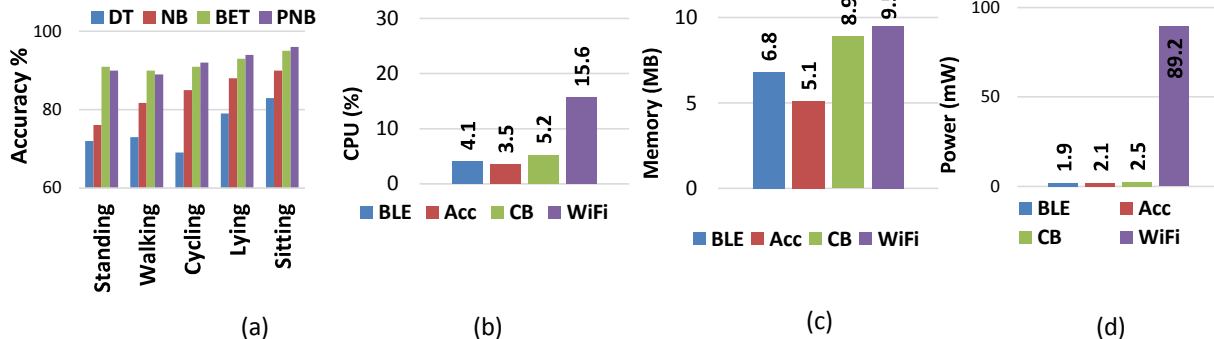
Figure 11: (a) Low-level activity recognition accuracy and (b) CPU utilization (%) (c) Memory Usage (MegaBytes) and (d) Power Consumption (miliWatt) measure for Bluetooth Low Energy (BLE), Accelerometer (ACC), Classical Bluetooth (CB) and WiFi
