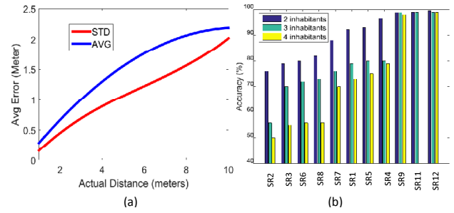
Figure 10: (a) iBeacon distance accuracy (b) Trilateration based localization accuracy for each sub-region (sorted by area)
