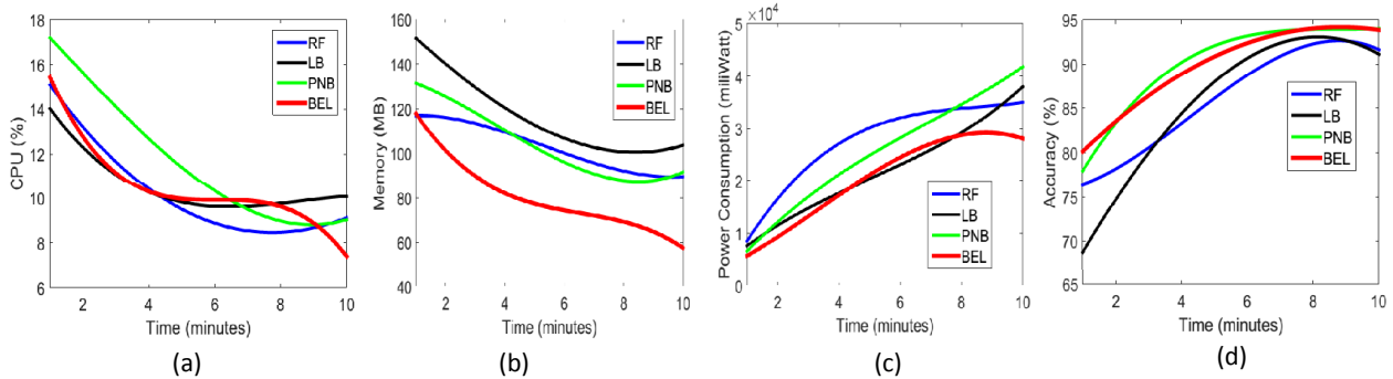
Figure 12: (a) CPU utilization (%) (b) Memory Usage (MegaBytes) and (c) Power Consumption (miliWatt) (d) Accuracy measure for Bagging Ensemble Learning, RandomForest, LogitBoost and Packaged Naive Bayes classifiers
