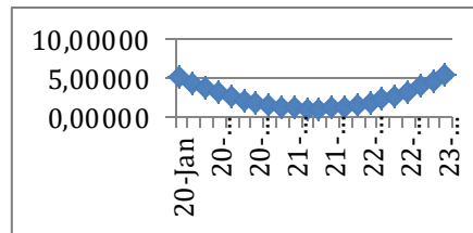
Fig. 2. Graph of GDP with Moderate Lockdown (ML) Source: Analysis, 2020
