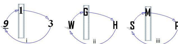
Fig. 1. Reflexivity Of 19 Source: Analysis, 2020
