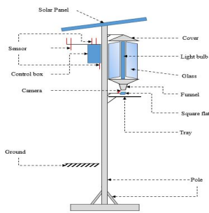
Figure 1. An automatic light trap
