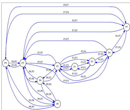
Figure 10. The logical network for the automatic light traps in Hau Giang
