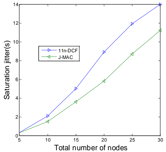
Fig. 6 Saturation jitter
