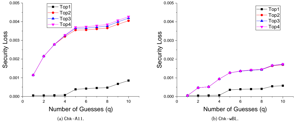
Figure 1. Security loss measured for different checkers and query numbers. Note that the security loss for Chk-A0p is zero, so we omit it for the sake of fin typogaphy.
