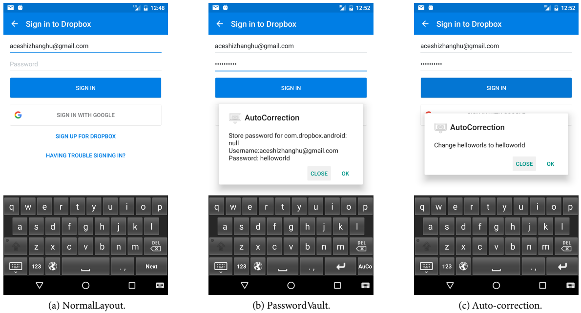
Figure 2. Screen-shots of a Dropbox login process. The pop-up dialogs are for the purpose of demonstration and do not appear in the real app.
