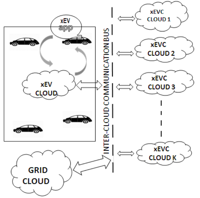
Fig.6. Communication interfaces among Federated Clouds
