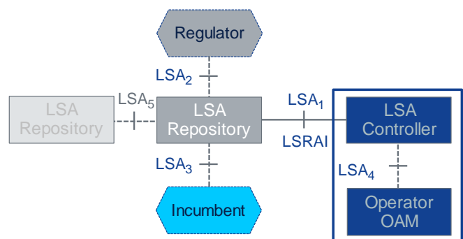
Figure 3. The LSA architecture reference model.
