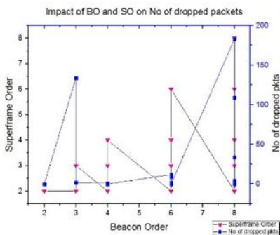
Figure 15. Number of Packets Drop vs BO and SO
