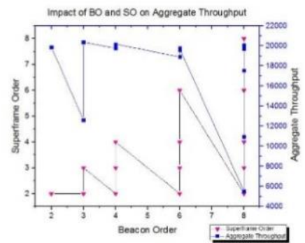
Figure 13: Aggregate Throughput vs BO and SO
