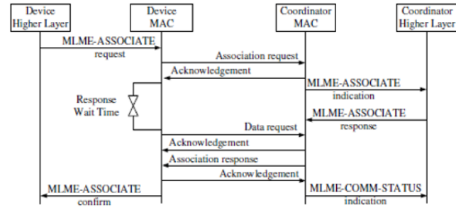
Figure 4: Nodes Association Process of IEEE 802.15.4 [10]
