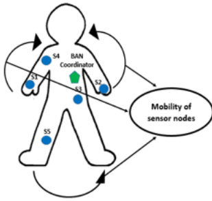
Figure 5: Mobility Scenario
