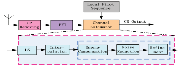
Fig. 6. The signal processing of the channel estimation module at the receiver.
