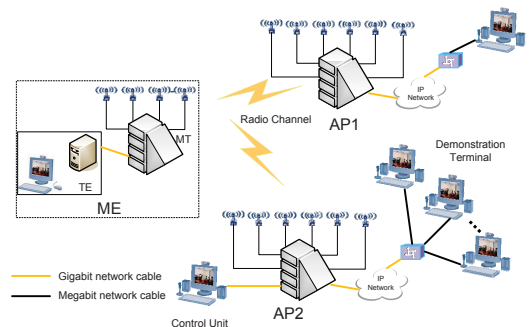
Fig. 9. Topology architecture of TDD-GBPS system.
