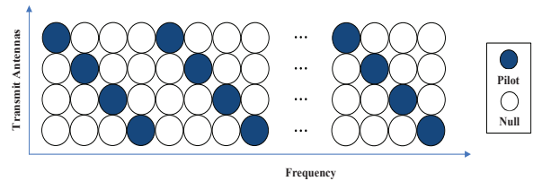
Fig. 3. Pilot pattern adopted in TDD-GBPS system.
