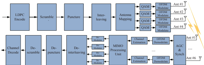
Fig. 1. Block diagram of TDD-GBPS uplink.
