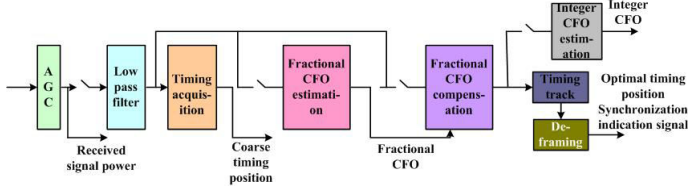
Fig. 4. The signal processing of the synchronization module at the receiver.
