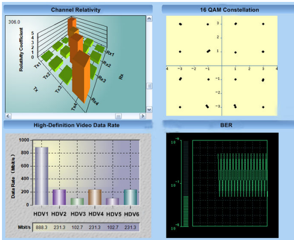
Fig. 11. Link-level transmission performance surveillance.
