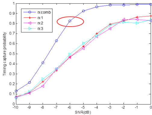
Fig. 5. Correct capture probability of synchronization.
