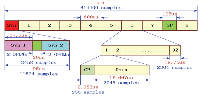
Fig. 2. The asymmetric frame structure.
