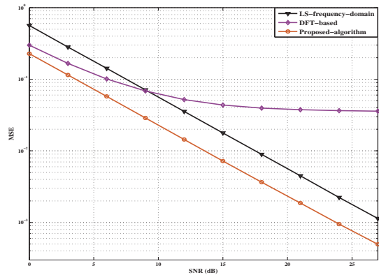
Fig. 7. MSE performance comparison.
