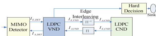
Fig. 8. The LDPC decoding architecture.
