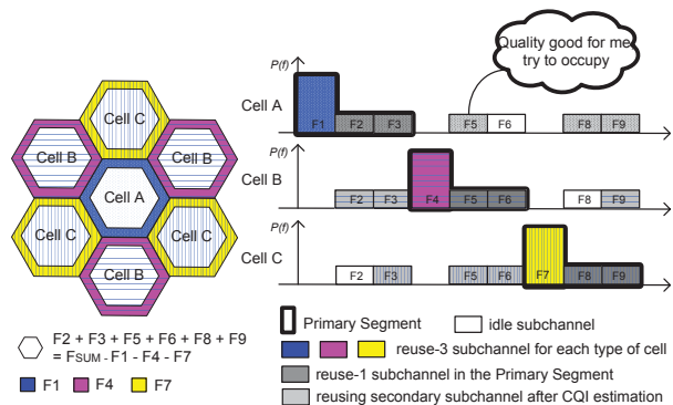
Fig. 4. Concept of the EFFR scheme in a cellular system based on partition of the exclusive reuse-3 subchannels and reuse-1 subchannels in the Primary Segment, as well as interference aware reuse on the Secondary Segment.
