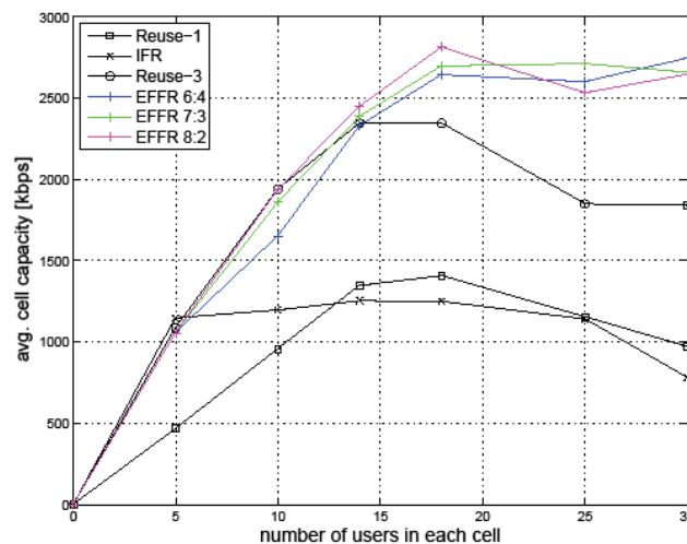
Fig. 6. Mean overall uplink cell capacity of four frequency reuse schemes as a function of the number of users in each cell, assuming users uniformly distributed over all cells in the system.
