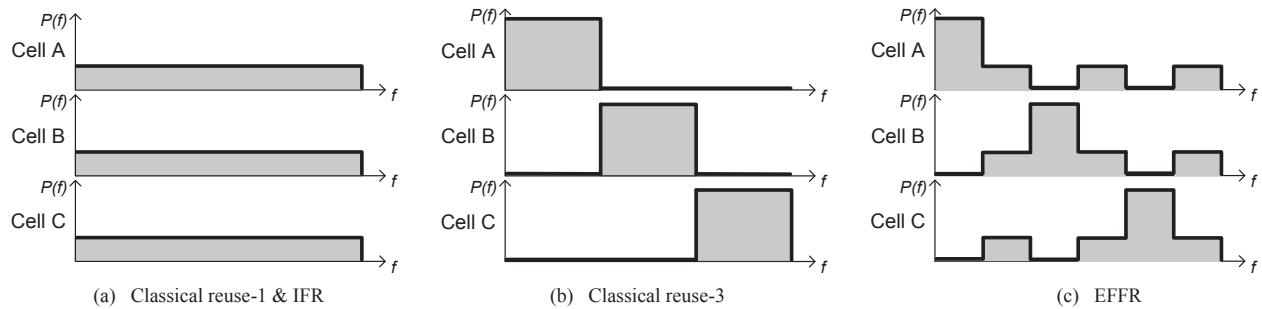
Fig. 5. Cell-specific power masks over system bandwidth for classical reuse-1, IFR, reuse-3 and EFFR.
