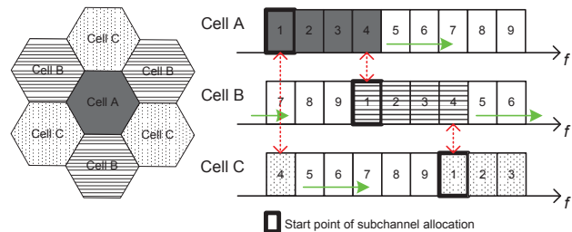
Fig. 3. Operation policy of the IFR scheme in a cellular system with 3 various types of neighboring cells.
