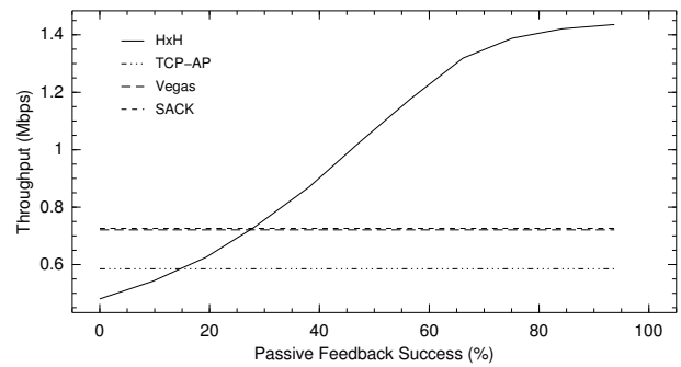
Figure 9: HxH Throughput vs Passive Feedback Success Rate
