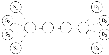
Figure 3: Dumbbell Topology
