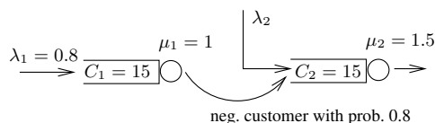
Figure 2: A network with negative customers.
