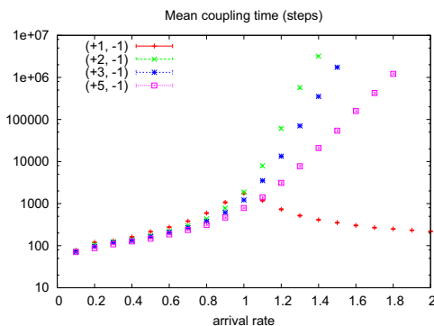
Figure 5: Mean coupling times for EPSA in a (+k, -1) queue with batch arrivals of size k = 1, 2, 3 and 5 respectively, as a function of the arrival rate \lambda .
