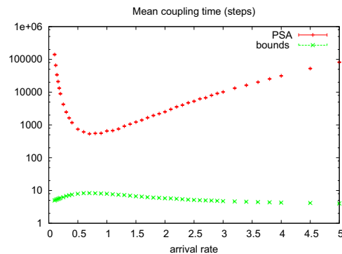
Figure 8: Exact values versus bounds for a (+4, -3) queue.
