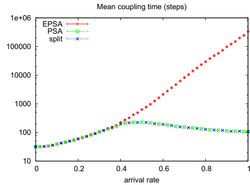
Figure 7: Mean coupling times for PSA, EPSA and EPSA with splitting for a (+2, +3, -1) queue.
