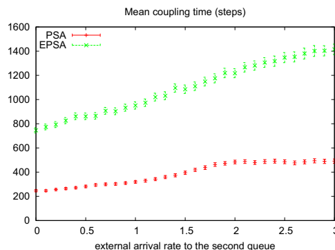
Figure 3: Mean coupling times of PSA and EPSA algorithms for the network in Figure 2 as a function of \lambda_2 .
