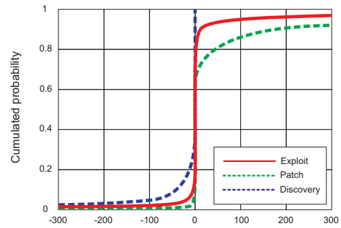
Figure 5: Probabilities before disclosure
