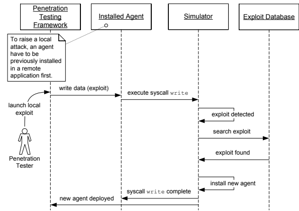
Figure 3: Local attack model.
