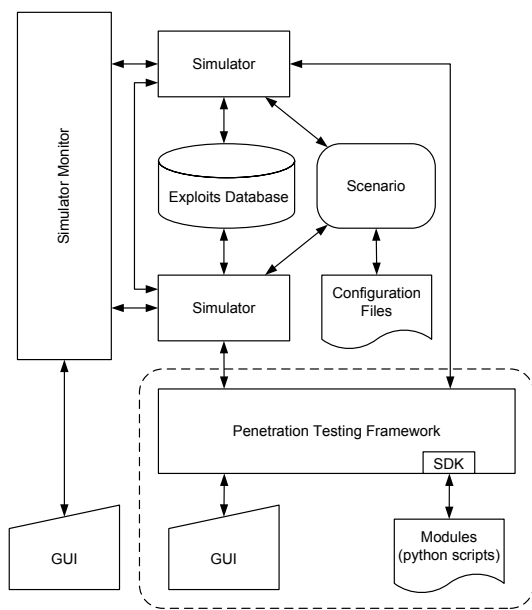
Figure 1: Insight architecture layout.
