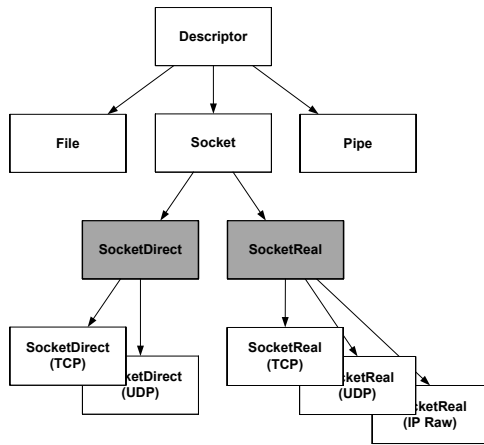
Figure 4: Descriptors' object hierarchy tree.
