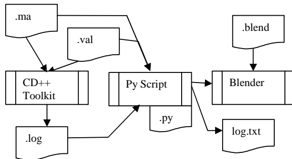
Figure 3: Visualization Architecture
