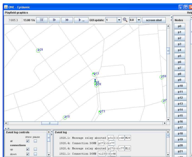
Figure 2: Screenshot of the ONE simulator's GUI
