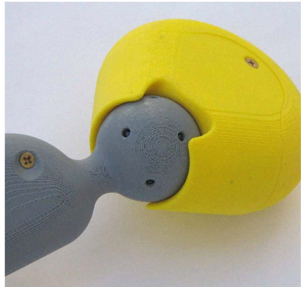
Fig. 1. Detail of optocoupled ball and socket joint of Posey construction kit.
