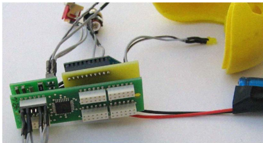
Fig. 4. Hub electronics includes an ATmega168 chip, Li Ion battery and charger circuit, Xbee radio transceiver, and connectors for four phototransistors (not shown) for each socket.
