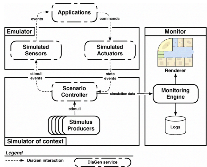
Fig. 7. The DiaSim simulator architecture
