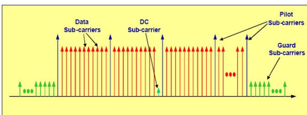
Figure 1. OFDM Sub-Carrier Structure [4]
