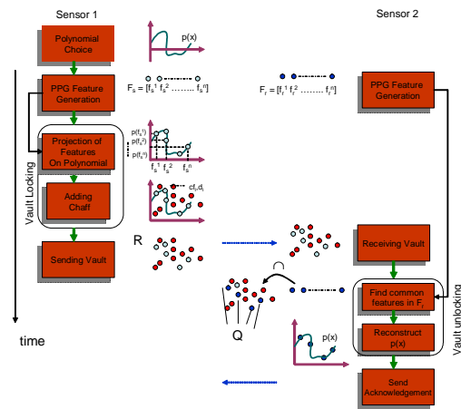
Figure 2: Key Agreement with PKA Protocol [24]
