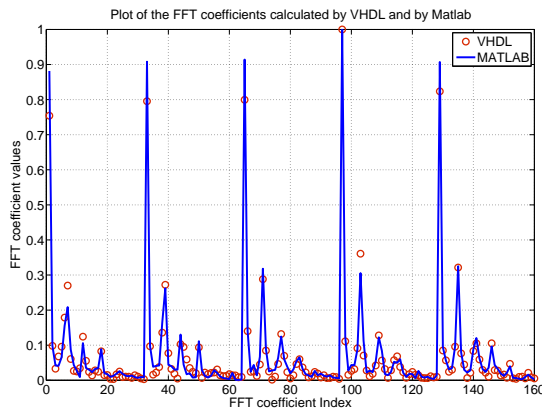
Figure 6: Comparison of FFT coefficients computed by VHDL and Matlab
