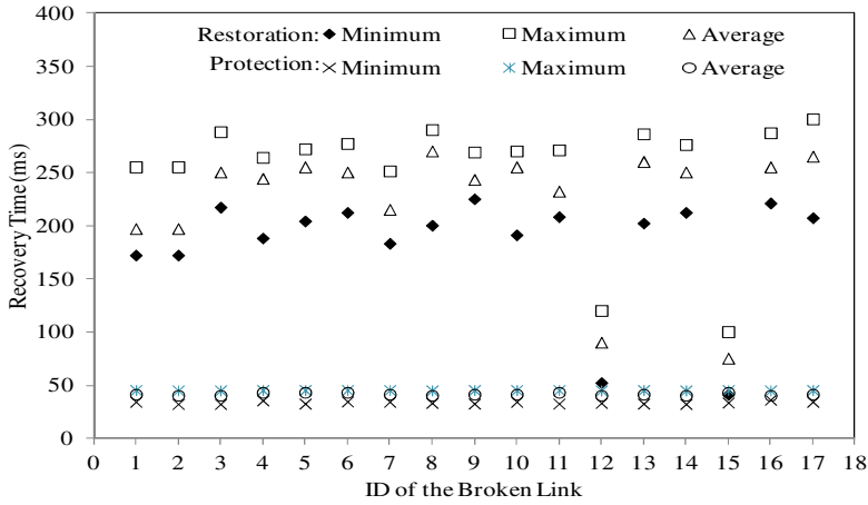
Fig. 2. Recovery Experiment
