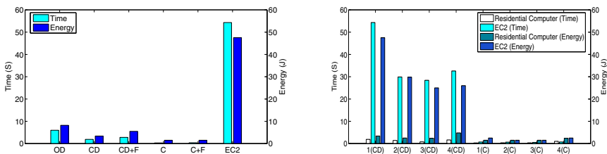
(a) Response Time and Energy Consumption (b) Response Time and Energy Consumption for Parallel Processing
