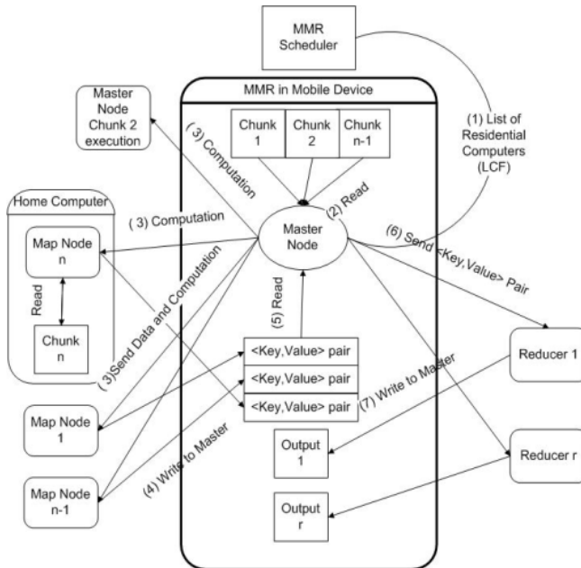
Fig. 3. MapReduce and MMR
