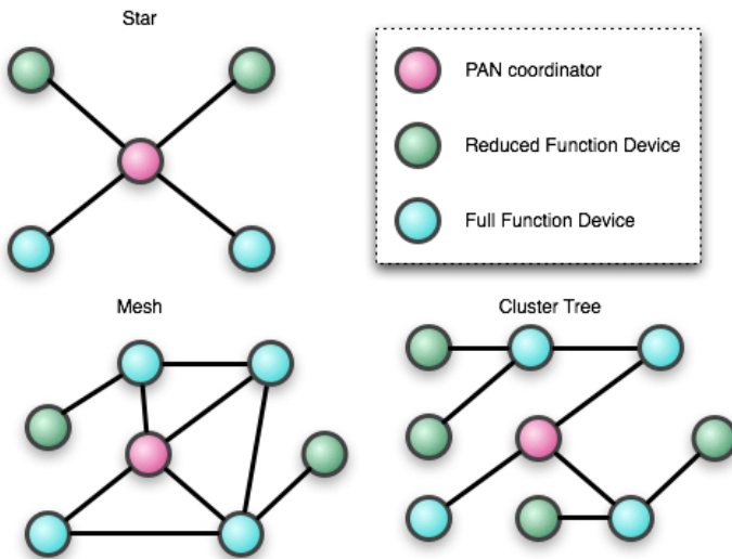
Fig. 4. Zigbee topologies
