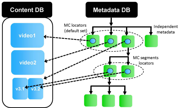
Fig. 5. Hierarchical MPQF model
