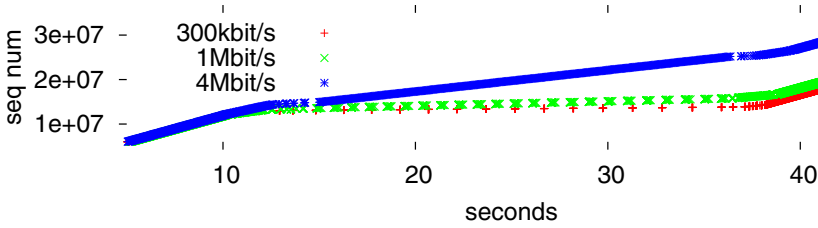
Fig. 5. Handover scenario with various WWAN bandwidth and (10Mb/s, 10ms) WLAN
