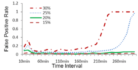
Fig. 5. False positive rate over time for different percentages of malicious verifiers. The claim generation rate is 1 per minute and the average speed is 1m/s.
